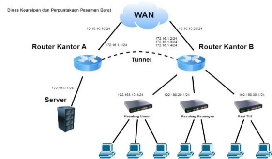
Figure 1. VPN + L2TP Network Topology
