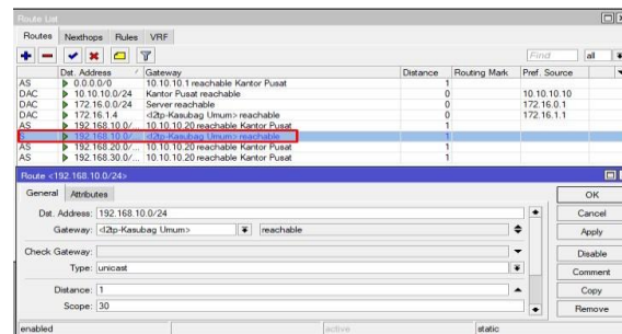
Figure 6. Result Of VPN L2PT Configuration
