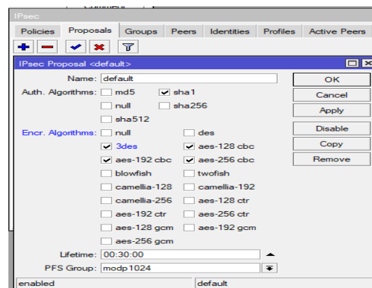
Figure 5. IP Sec Configuration
