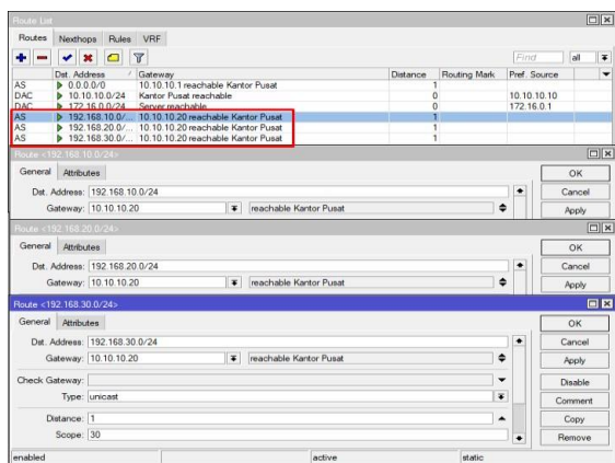
Figure 3. Routing Router A
